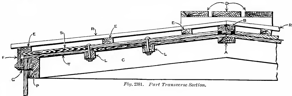
Fig. 2380. Part Transverse Section.
